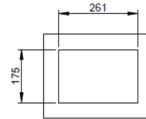
Recommended cutout
